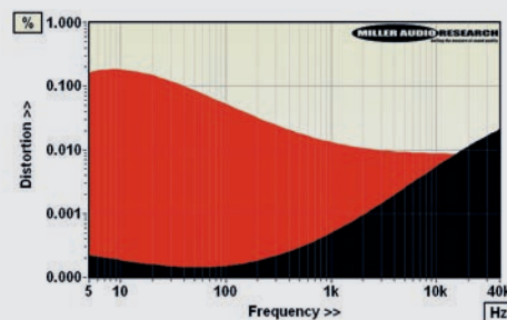
ABOVE: Distortion vs. extended 5Hz-40kHz frequency (black, Pre Box at 0dBV; red, Amp Box at 1W/8ohm)
