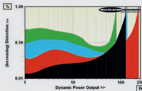
ABOVE: Dynamic power output versus distortion into 8ohm (black), 4ohm (red), 2ohm (blue) and 1ohm (green) loads. Maximum current is 8.9A
